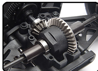
Metal gear transmission with sealed metal gear differentials
